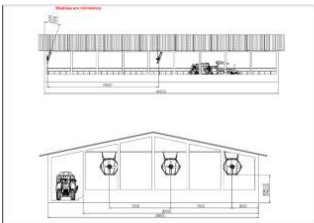
Figura 2 - Layout compost barn
